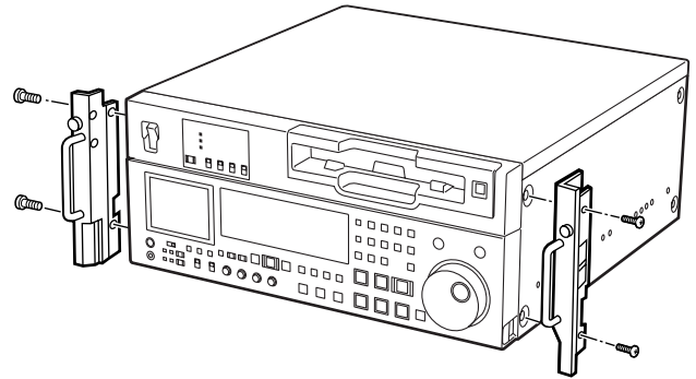
Rack-mounting adaptors
