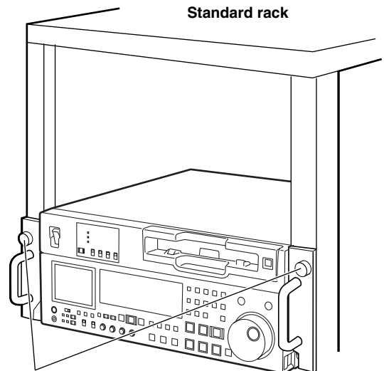
Fasten it to the rack with set screws.
